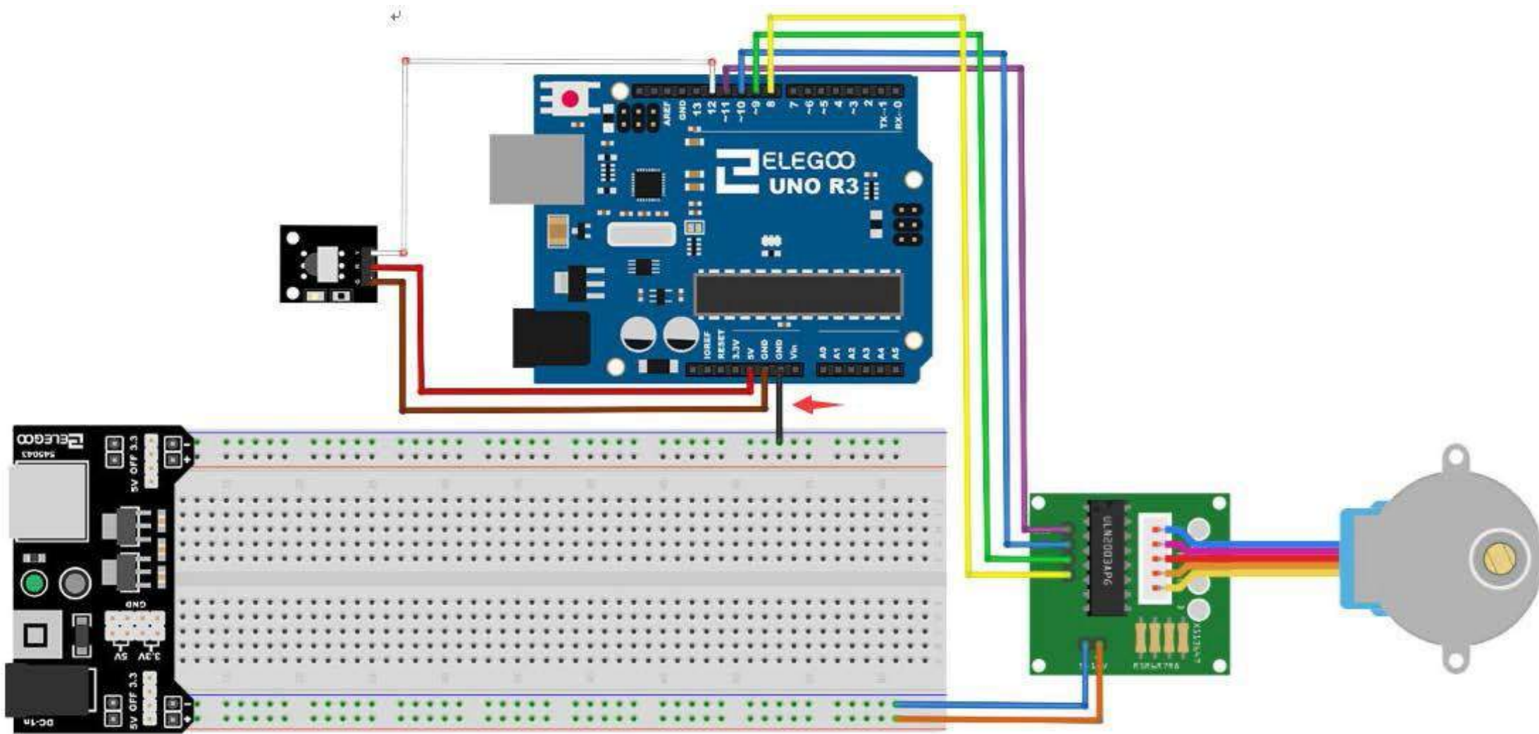
Wiring diagram
